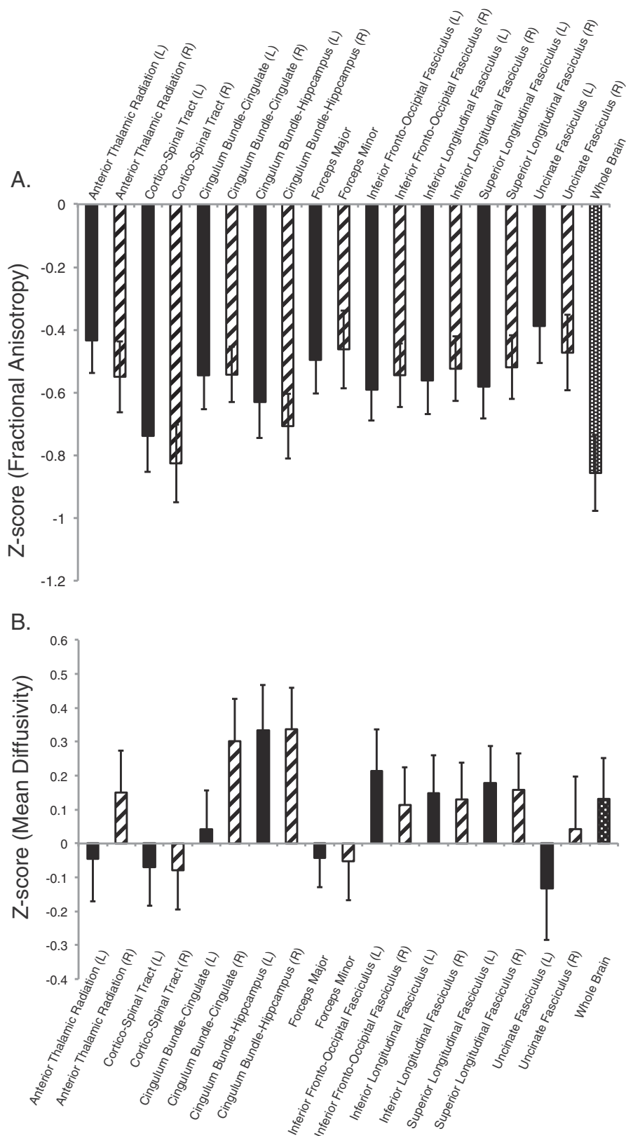
Fig. 8. Normalized (z-transformed) regional (A) FA and (B) MD values in Poor data. ROI data from ICBM-JHU White Matter Atlas. Data are normalized data that passes QA.
