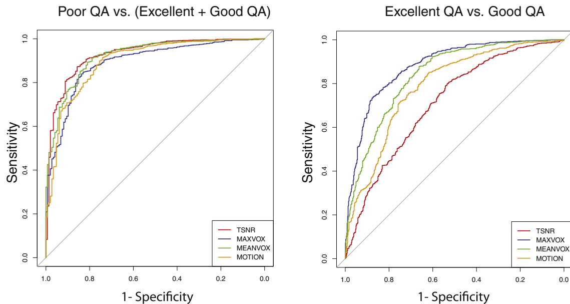
Fig. 4. Receiver–operator characteristic curves of TSNR, MAXVOX, MEANVOX, and MOTION. (A) ROCs for differentiating Poor data from acceptable data (Good + Excellent). TSNR best differentiated Poor data from acceptable data. (B) ROCs for differentiating excellent data from Good data. MAXVOX best differentiated excellent data from Good data.
