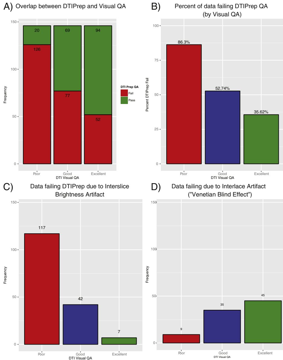
Fig. 10. Comparison of DTIPrep QA with our Visual QA methods. The two methods were in the highest agreement for Poor data followed by Good then Excellent. However, DTIPrep at the default setting considered more data to fail.
